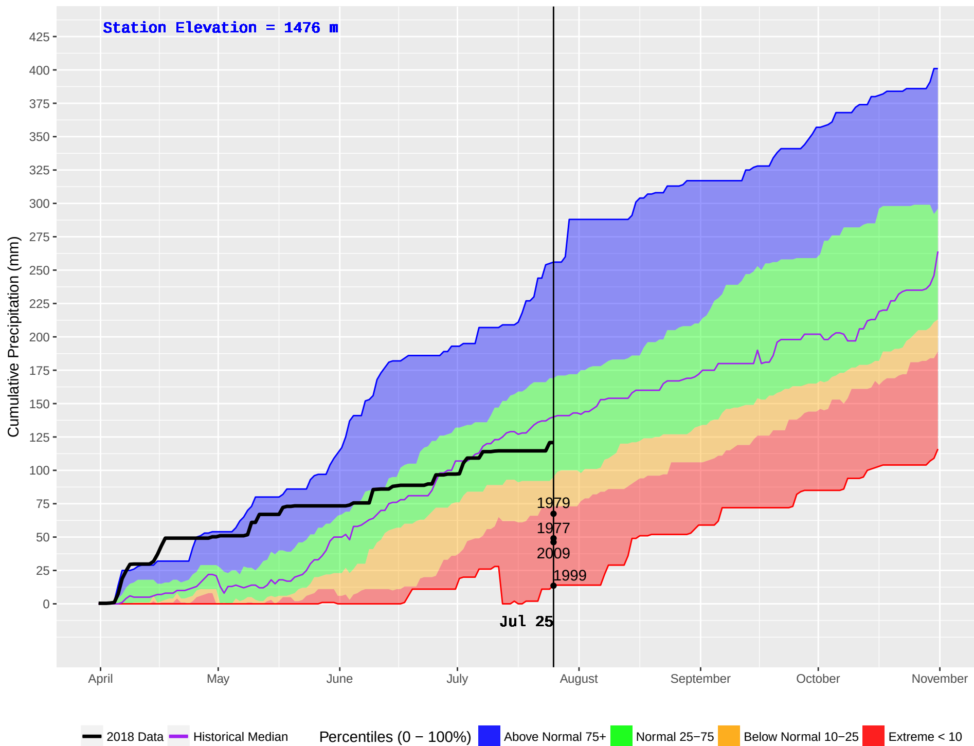
BRENDA MINES (283) : Historical (1977–2016) and Current (2018) Noon Cumulative Precipitation
