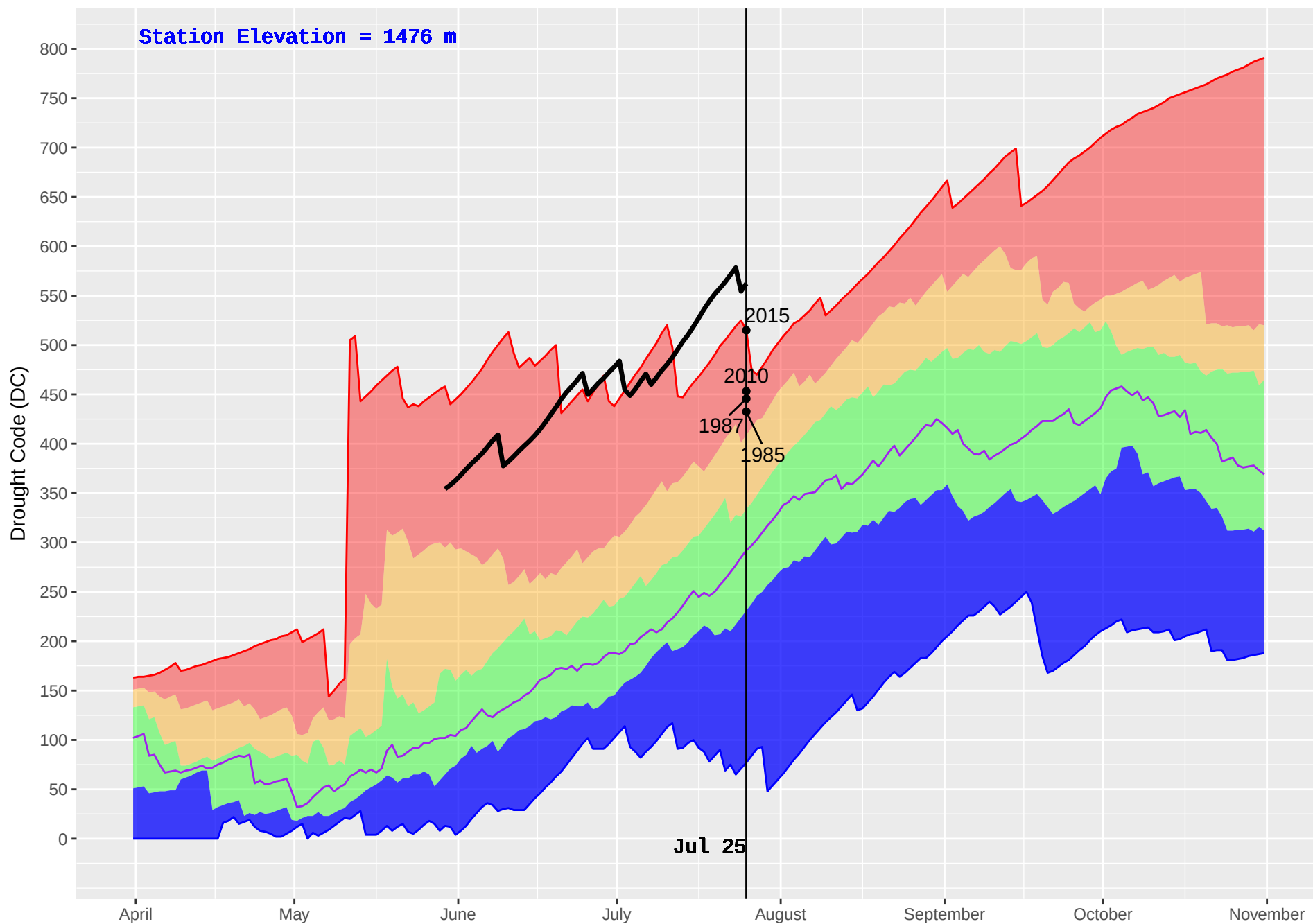
BRENDA MINES (283) : Historical (1977–2016) and Current (2018) Noon Drought Code (DC)
